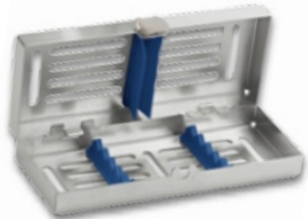
12-147-06 For 5 instruments 182x72x34mm
